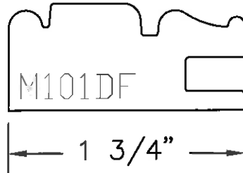
Drawer Front Profile
